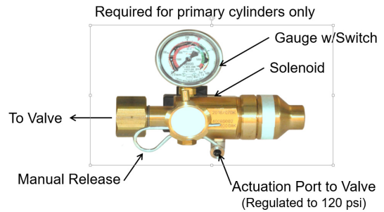
Figure 5. Release Unit
