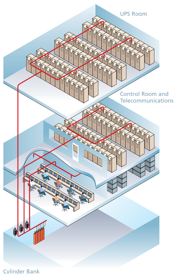
Typical Argonite system protecting separate spaces from the same cylinder bank.
